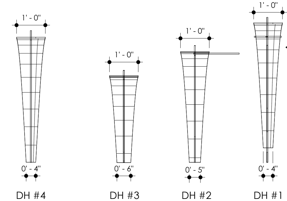
4 DECORATIVE HORNS/ FRONT VIEW 1/2" = 1'-0"
