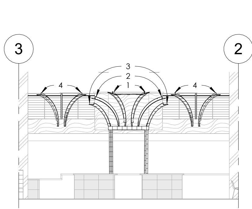
1 DECORATIVE HORNS ELEVATION 1/8" = 1'-0"
