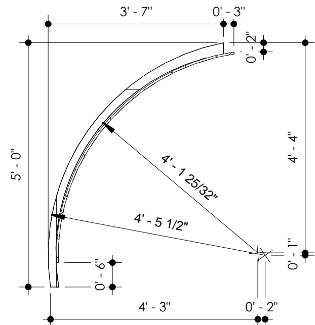
4 DECORATIVE HORNS/ FRONT VIEW 1/2" = 1'-0"
