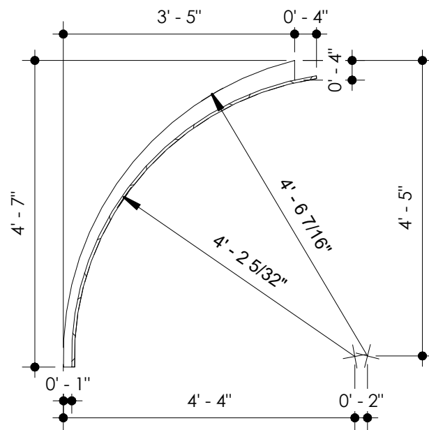
4 DECORATIVE HORNS/ FRONT VIEW 1/2" = 1'-0"
